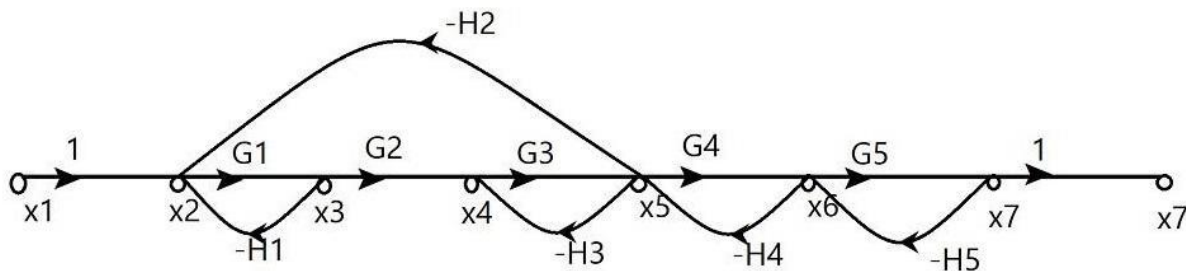
Signal Flow Graph
