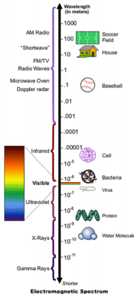
Figure 3 Electromagnetic spectrum
