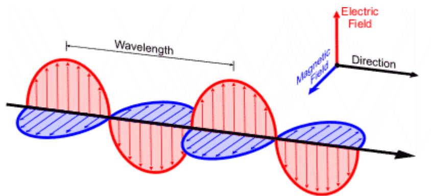
Figure 2 Electromagnetic waves
